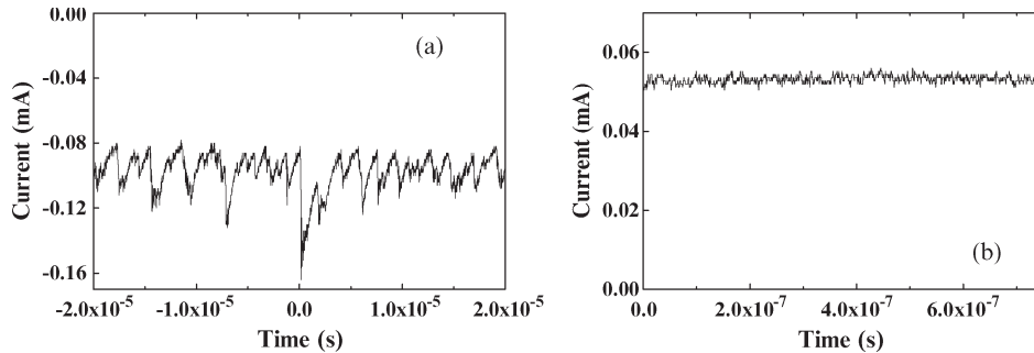
Fig. 2. (a) Negative and (b) positive corona current waveforms in atmospheric air at 0.3-bar gauge. The stress voltage: (a) -26 kV and (b) +26 kV.
