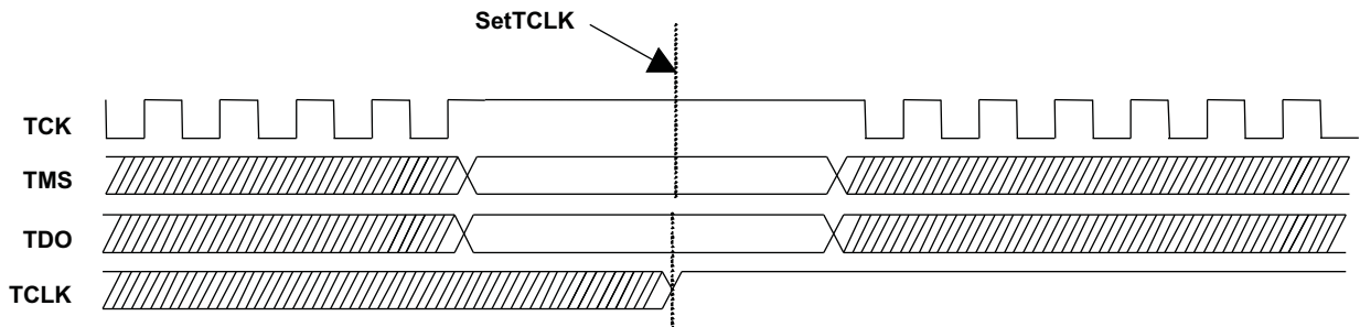
Figure 1-5. SetTCLK
